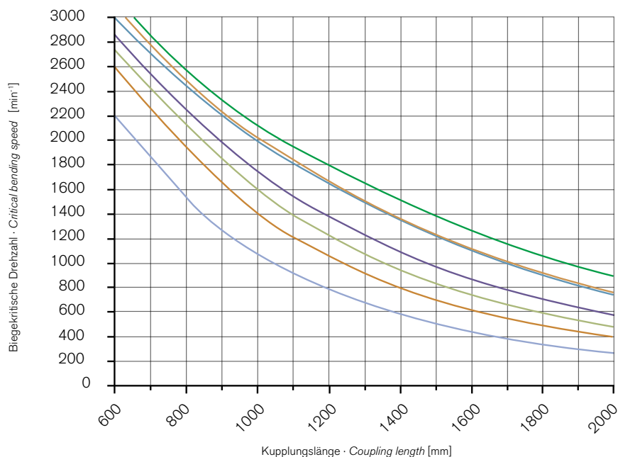
GWZ 5104.1
