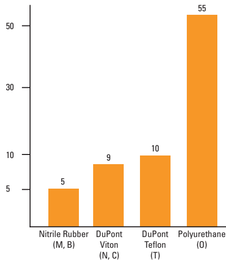
Fig. C-17. Relative abrasion resistance ratings.
