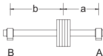
Fig. C-13. Overhung load.
